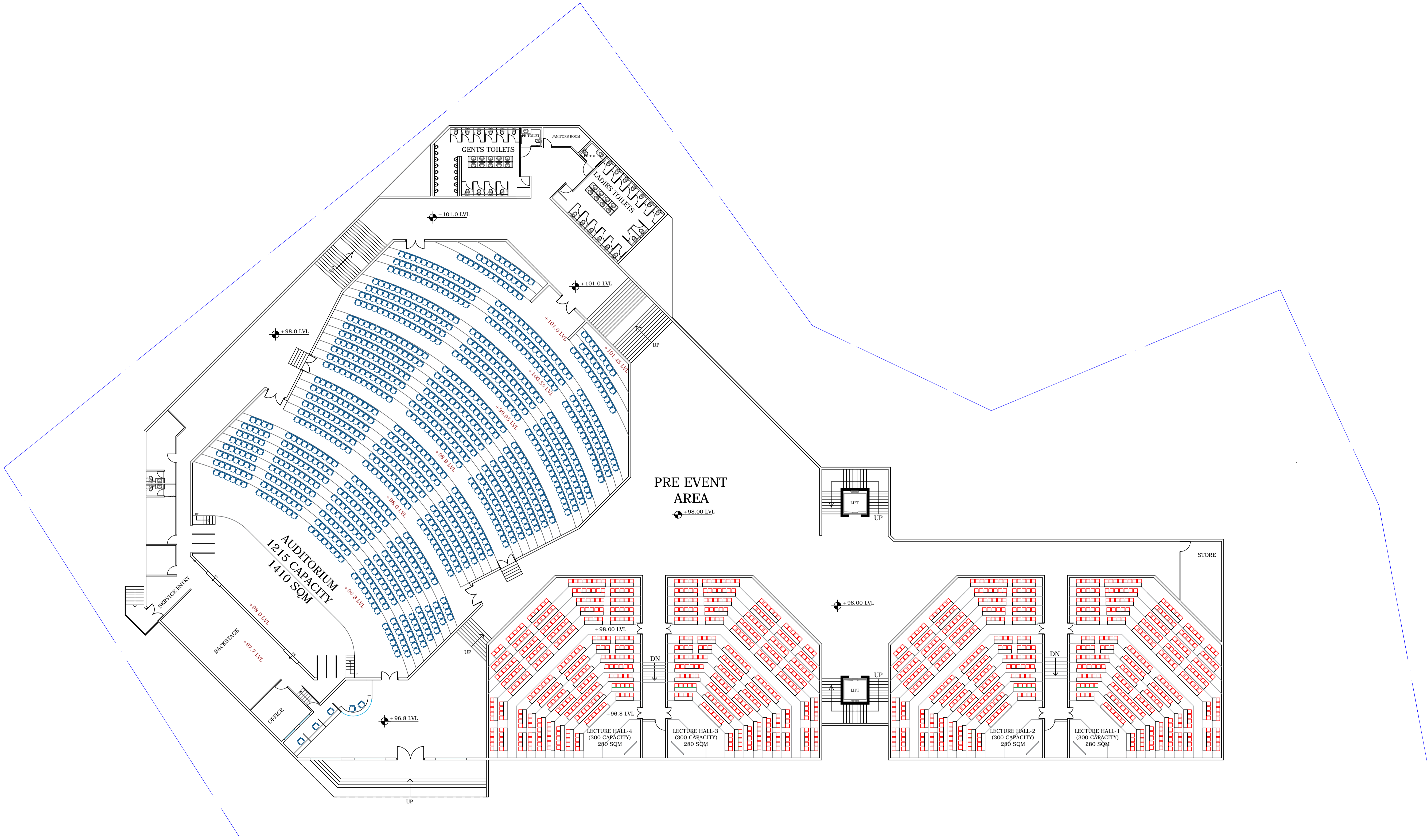
FLOOR PLAN @ +98.0 LVL FLOOR AREA= 4606 SQ M
